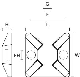
MCMB Mount (side and plan view)
