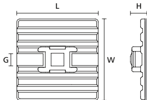
Flexible Mount with adhesive (plan view)
