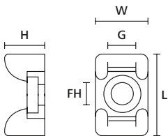
Cable Tie Mounts KR6G5, KR8G5 and CTM
